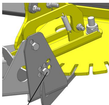
Vinkeljustering i 6 stillinger
